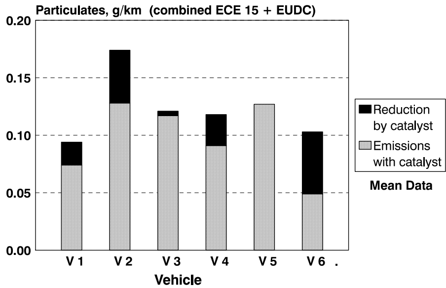
Figure 8 Average reduction of particulate emissions with oxidation catalyst in operation (low sulphur fuels)
