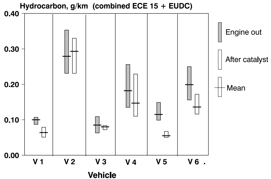
Figure 6 Hydrocarbon emissions (engine out vs. after catalyst) Levels and spread with low sulphur fuels
