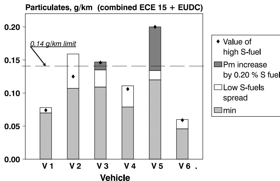
Figure 3 Effect of fuel sulphur on particulate emissions with oxidation catalyst
