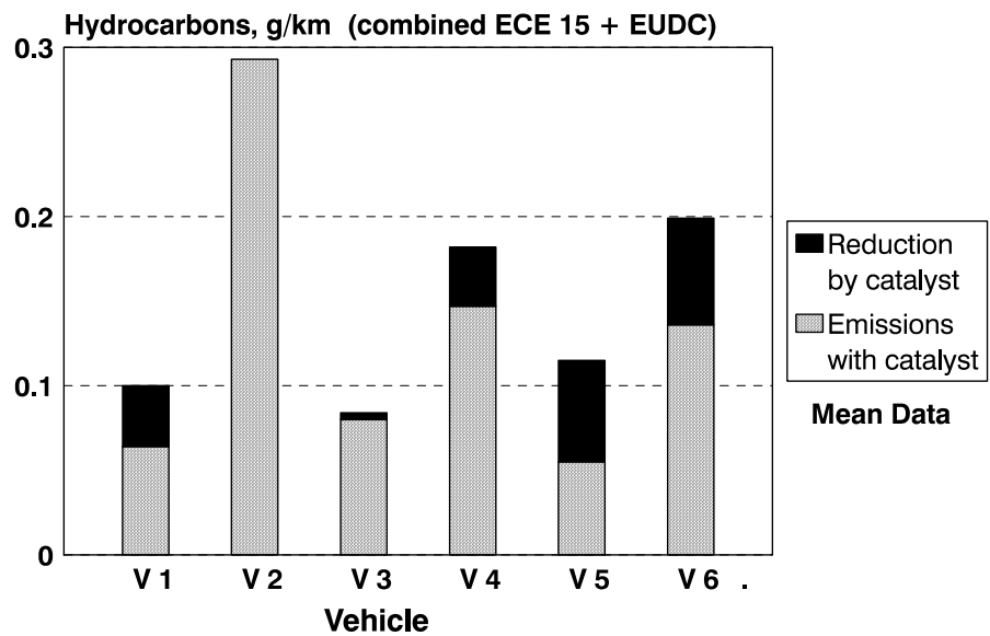
Figure 10 Average reduction of hydrocarbon emissions with oxidation catalyst in operation
