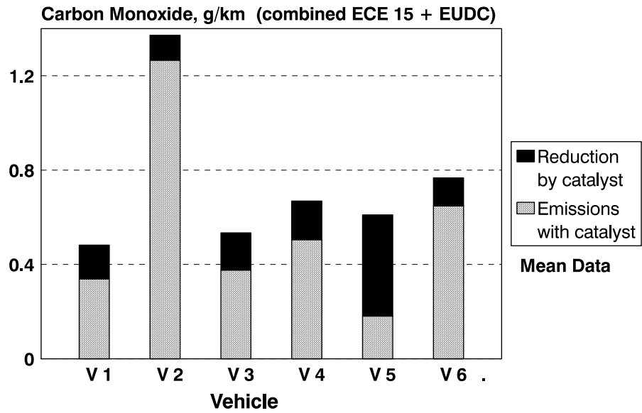
Figure 9 Average reduction of carbon monoxide emissions with oxidation catalyst in operation
