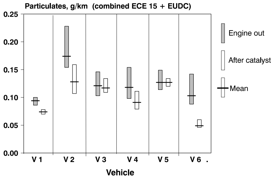
Figure 1 Particulate emissions (engine out vs. after catalyst) Levels and spread with low sulphur fuels
