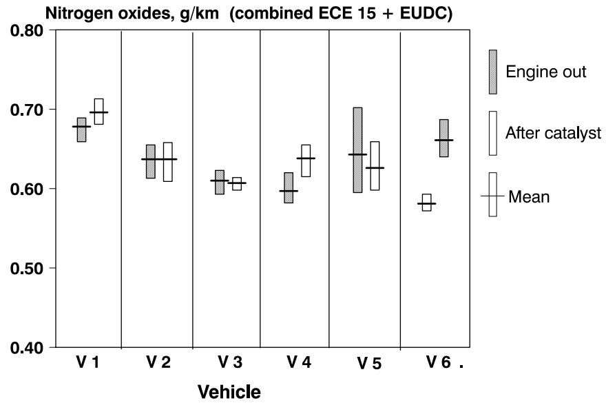
Figure 7 Nitrogen oxides emissions (engine out vs. after catalyst) Levels and spread with low sulphur fuels
