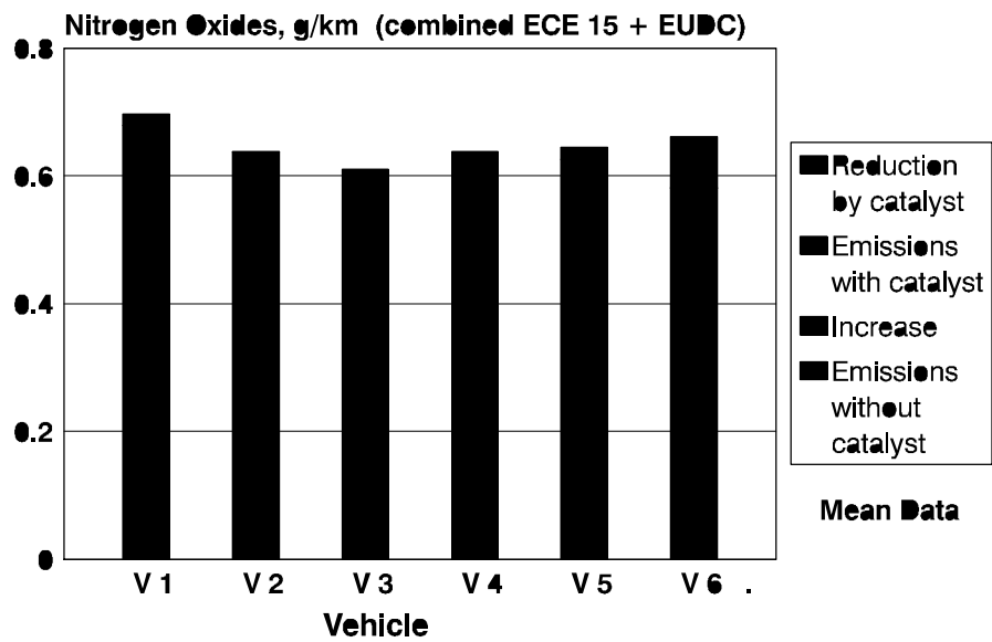
Figure 12 Average reduction of nitrogen oxides emissions with oxidation catalyst in operation
