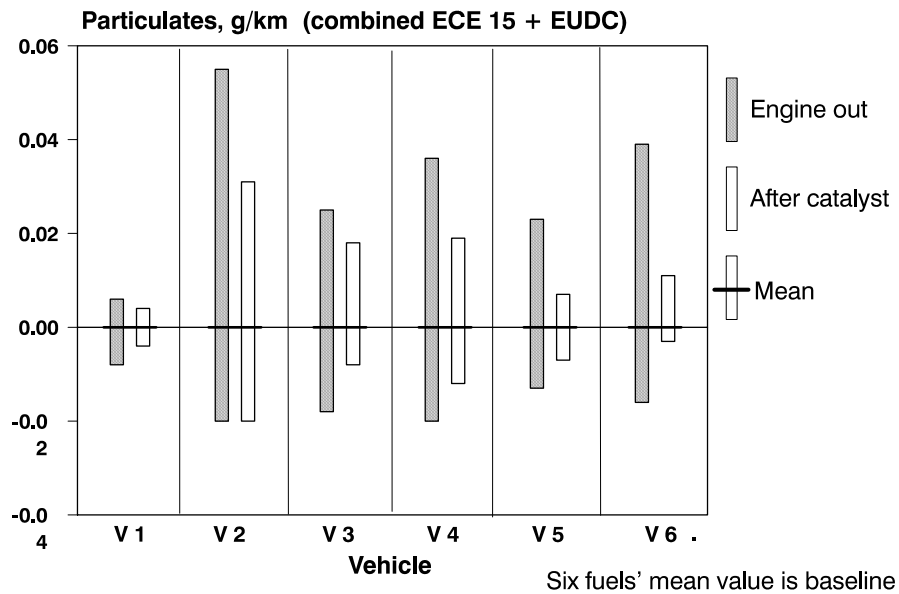
Figure 2 Particulate emissions spread (engine out vs. after catalyst) Low sulphur fuels
