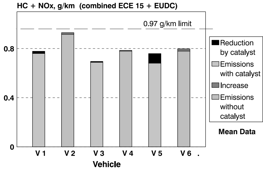
Figure 11 Average reduction/increase of HC + NOx emissions with oxidation catalyst in operation
