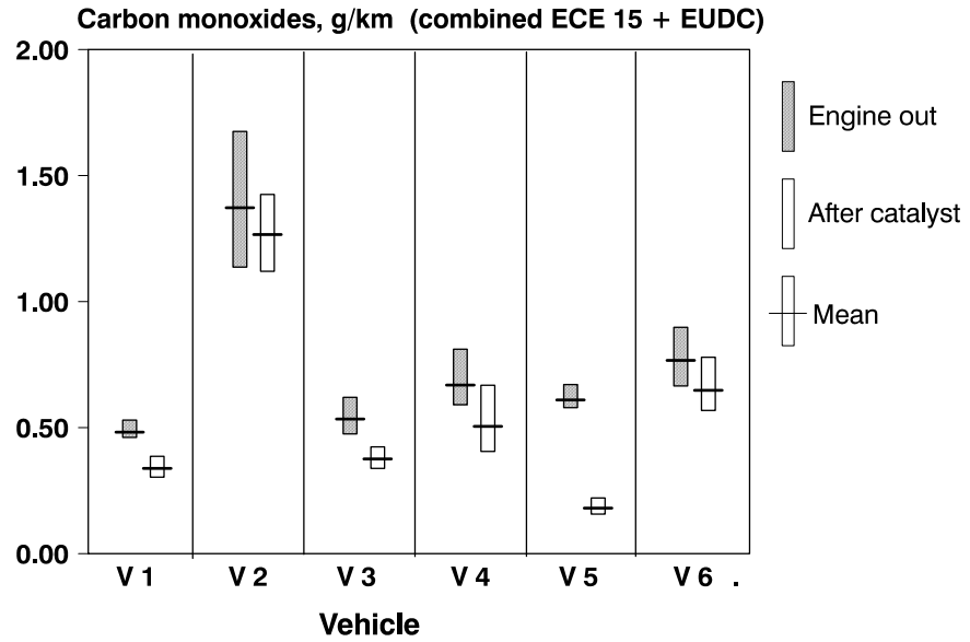
Figure 5 Carbon monoxide emissions (engine out vs. after catalyst) Levels and spread with low sulphur fuels
