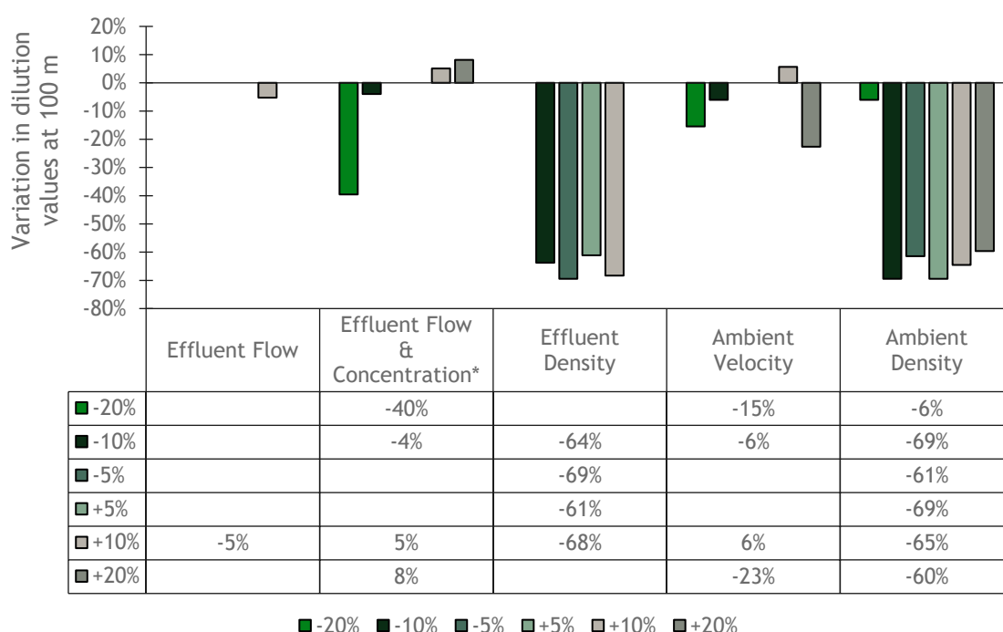
Figure 23. Discharge #4: Dilution values at 100 m
