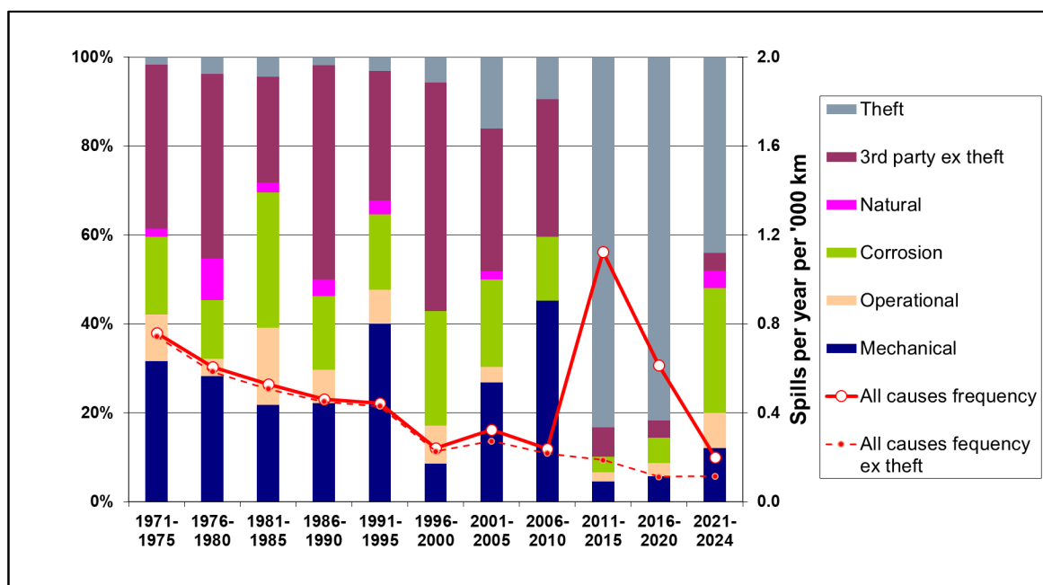
Figure 8a Cold pipelines spillage frequencies by cause Including theft
