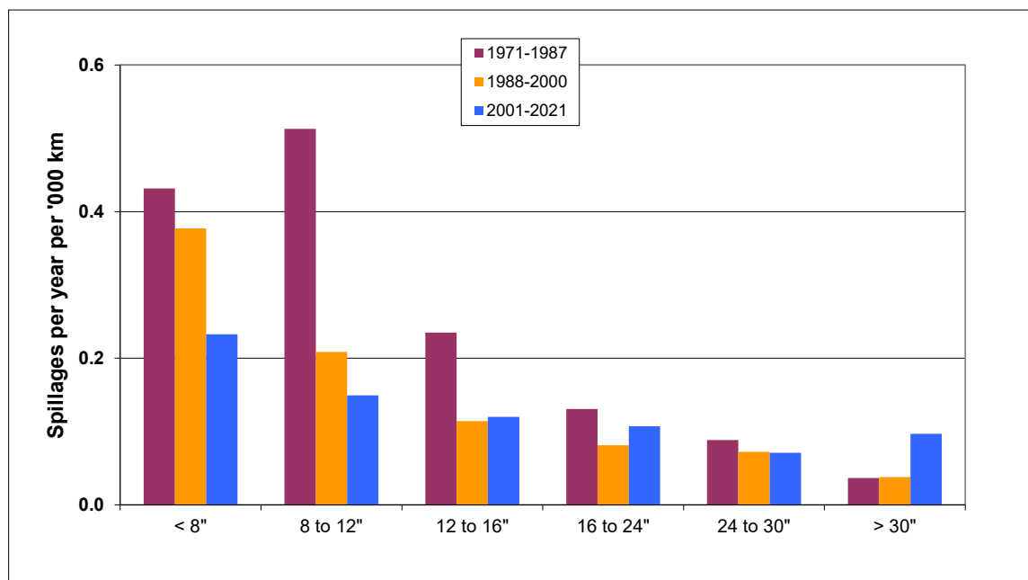
Figure 29 Third party accidental spillage frequencies per diameter class
