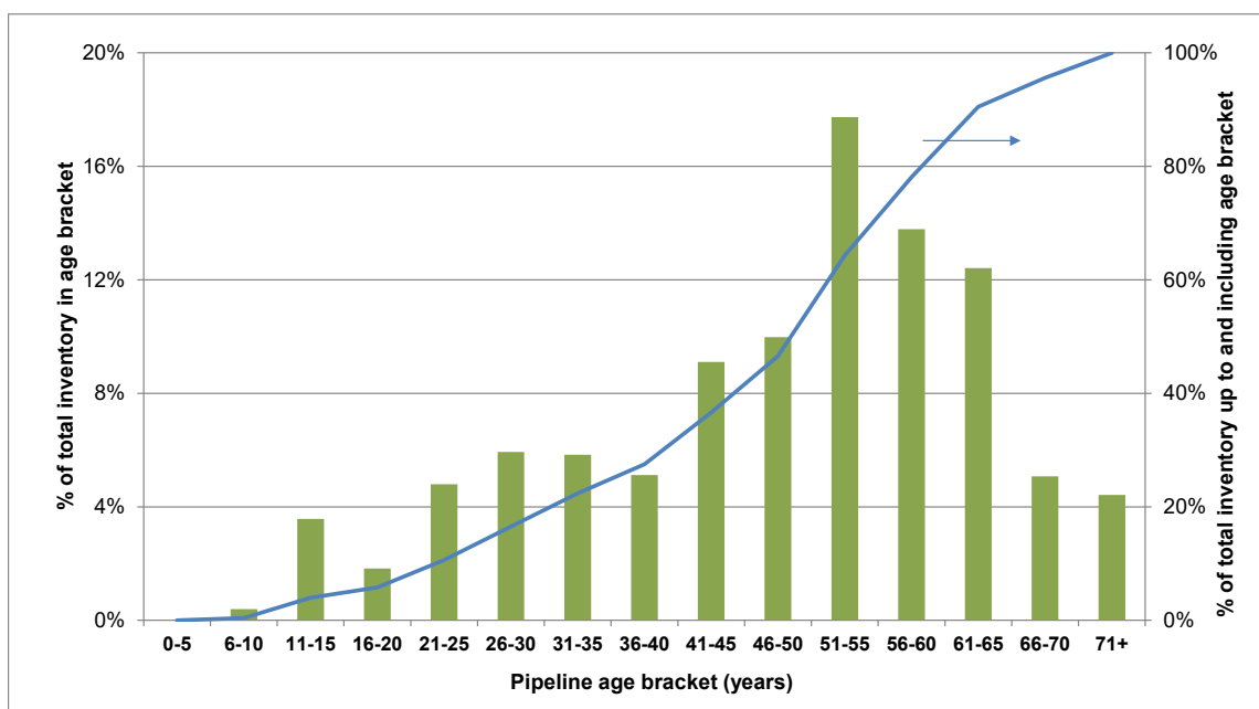
Figure 3b European Oil pipeline age distribution in 2021
