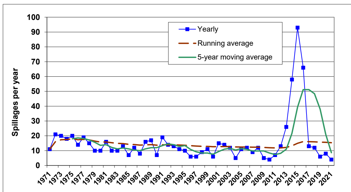
Figure 4a 51-year trend of the total annual number of spillages (all pipelines) Including theft
