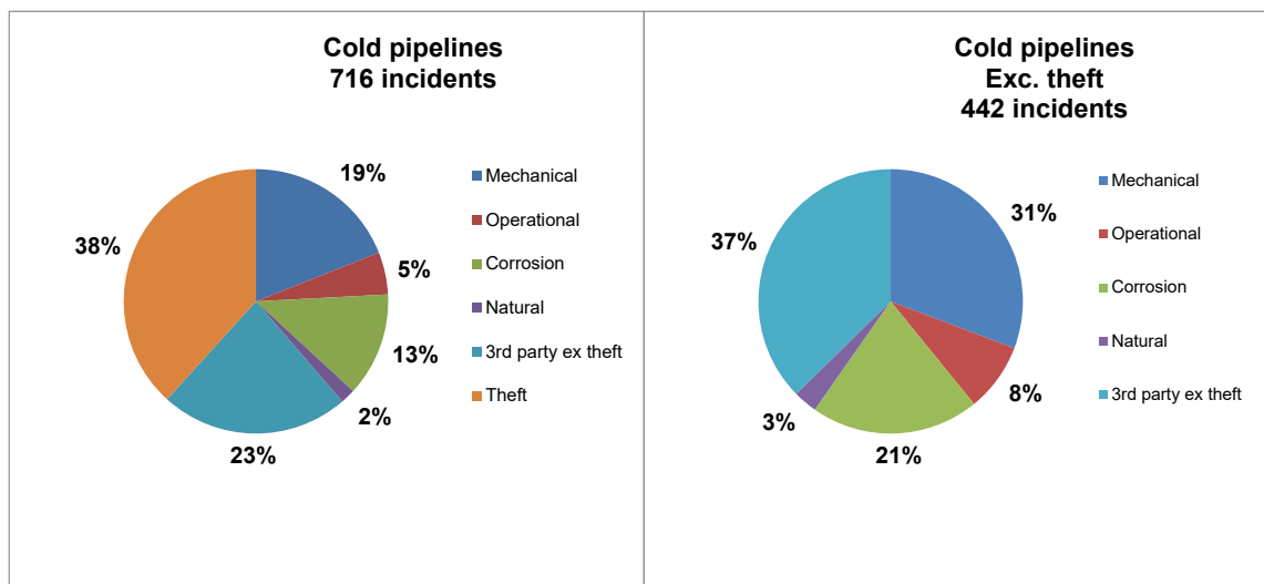
Figure 21 Distribution of major spillage causes for cold pipelines
