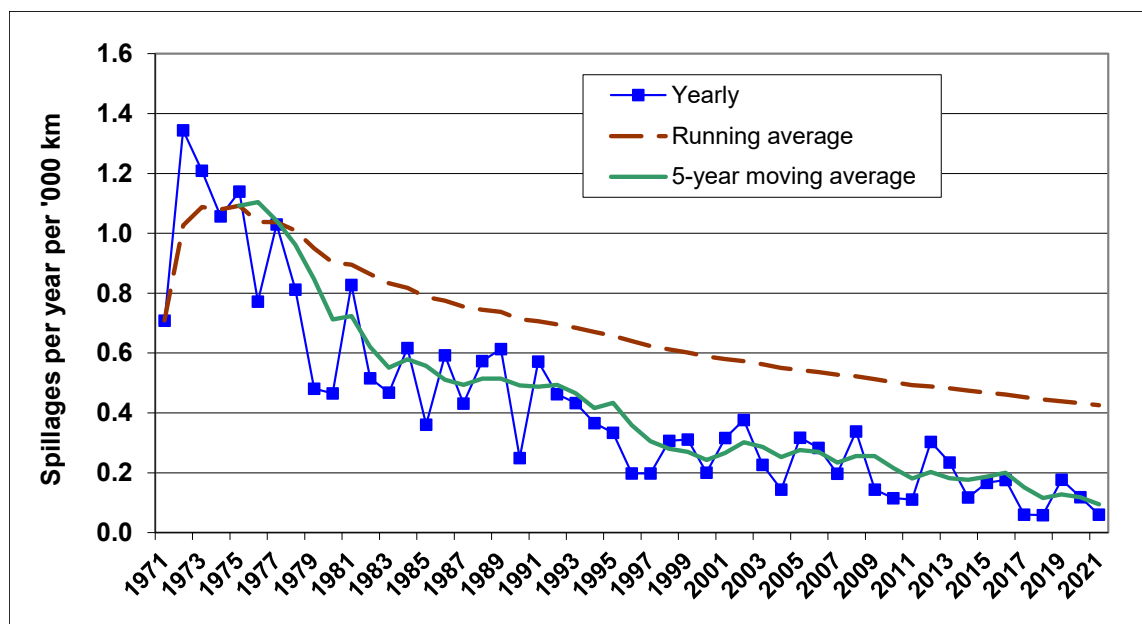
Figure 5b 51-year trend of the spillage frequency (all pipelines) Excluding theft
