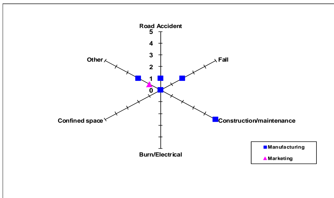
Figure 9 Causes of fatalities in 2011
