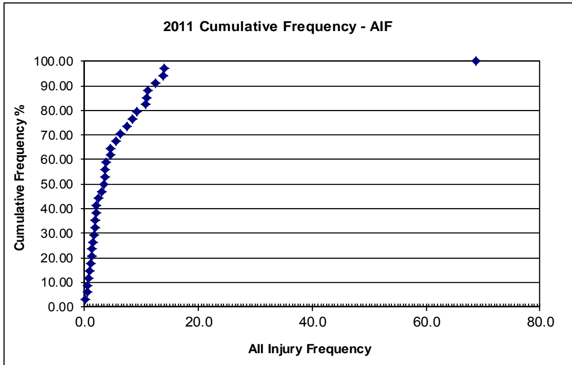
Figure 1b Cumulative Frequency Analysis All Injury Frequency
