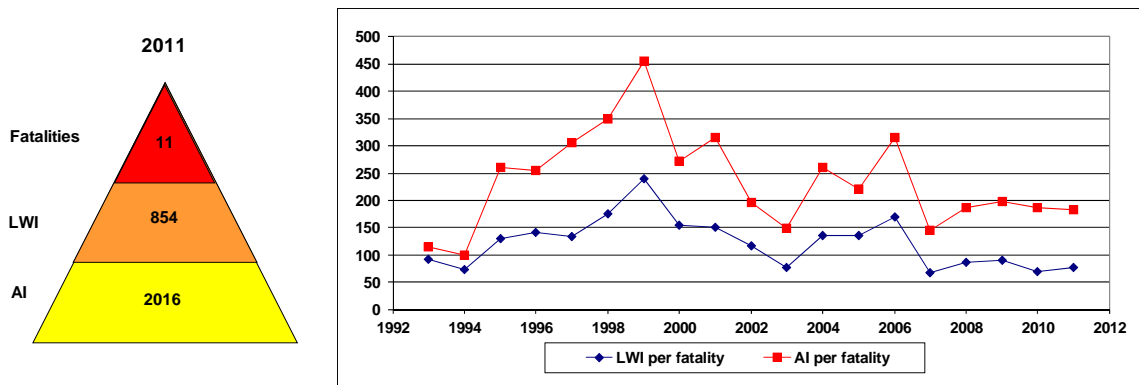
Figure 8a The safety triangle
