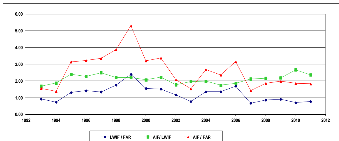
Figure 8b Relationship between the frequencies FAR, AIF and LWIF
