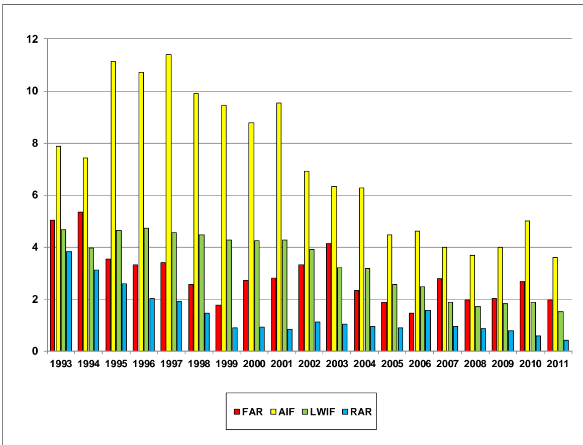
Figure 6a Historical evolution of main performance indicators Yearly data for the whole European downstream industry
