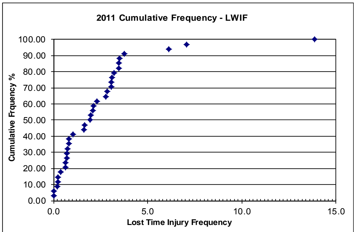
Figure 1c Cumulative Frequency Analysis Lost Work Injury Frequency
