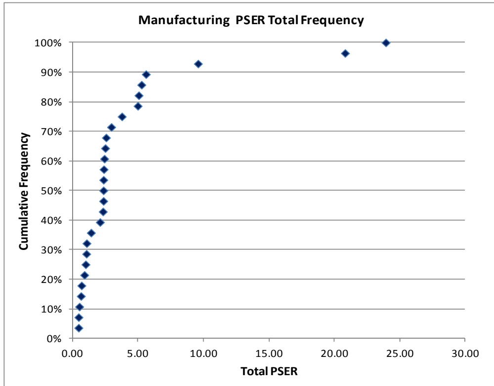
Figure 5b Cumulative frequency chart for Tier 1 Manufacturing PSER
