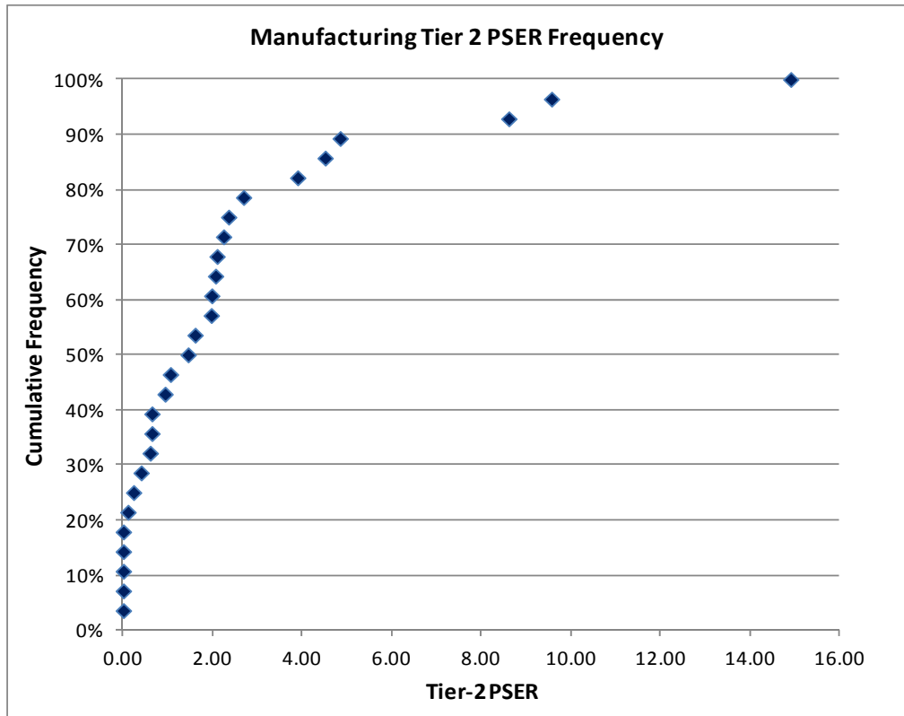
Figure 5c Cumulative frequency chart for Tier 2 Manufacturing PSER
