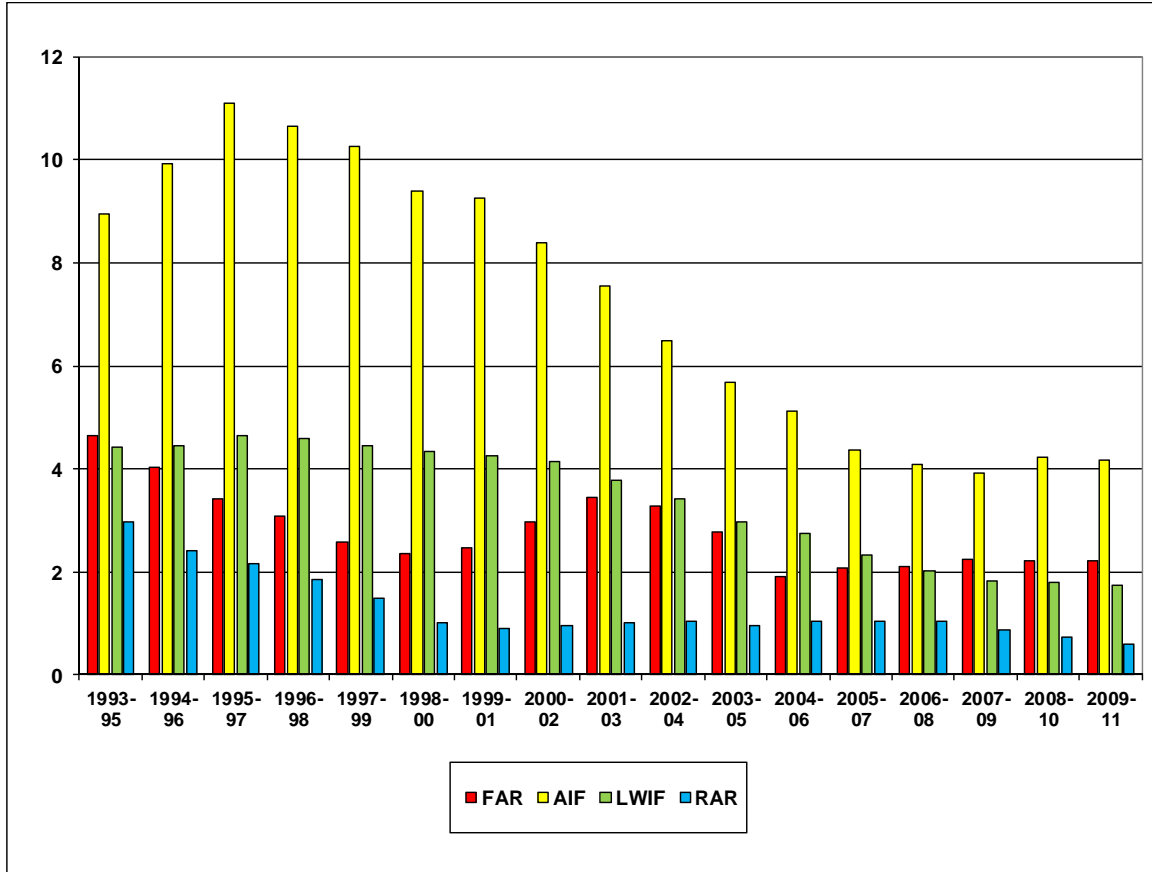
Figure 6b Historical evolution of main performance indicators 3-year rolling average for the whole European downstream industry
