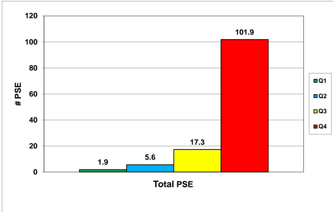
Figure 4b Total PSE distribution - Average value for each quartile
