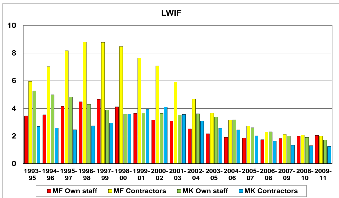
Figure 7b Historical evolution of Lost Work Injury Frequency segmented 3-year rolling average (MF: Manufacturing; MK: Marketing)
