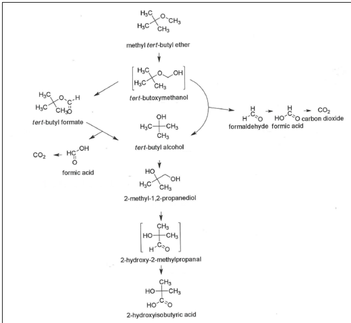
Figure 4.9 Reported aerobic biodegradation pathways to transform MTBE/TBA into HIBA (Debor & Bastiaens, 2007)
