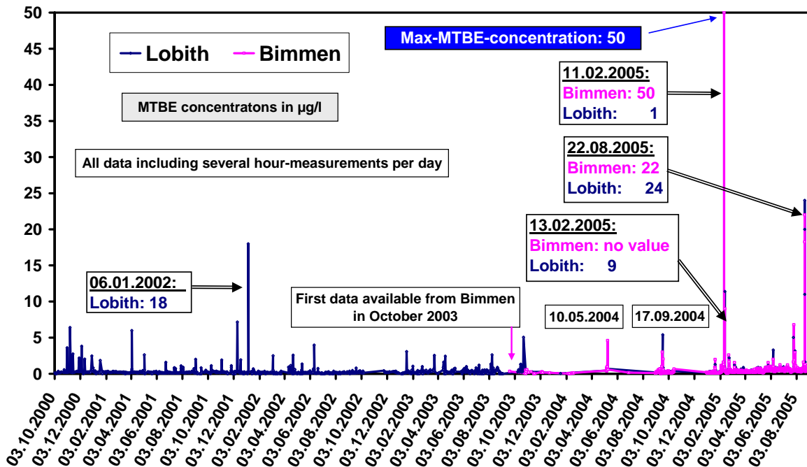
Figure 3.21 MTBE concentration (µg/l) in the River Rhine 2000 – 2005, based on data from monitoring stations Bimmen and Lobith
