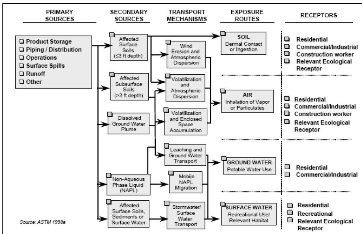
Figure 1.3 Example of an exposure pathway flowchart (after ASTM 1998)
