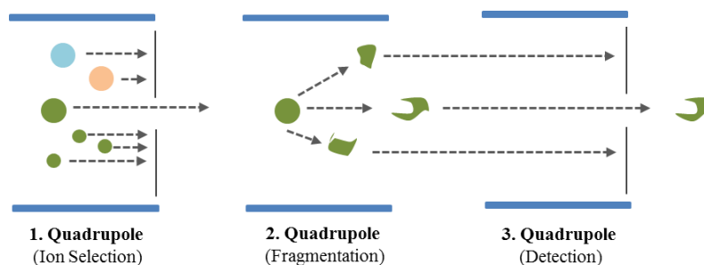
Figure 2. MS-MS-coupling principle
