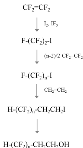
Figure 2.5: Production route of fluorotelomers via telomerisation (Buck et al., 2011)
